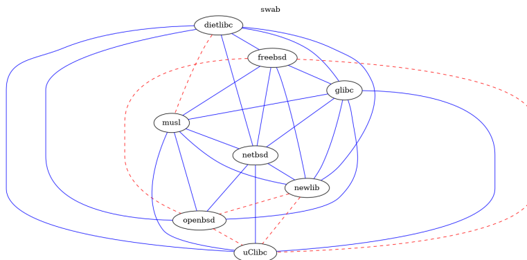
Figure 4.3: Equivalence Classes for swab
