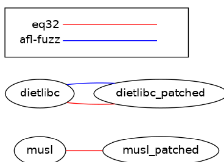
Figure 5.2: swab : An edge indicates that we were able to find a distinguishing input
