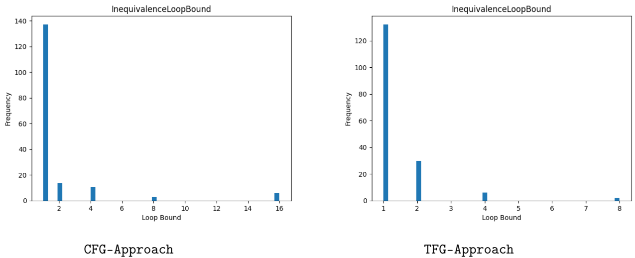
Figure 6.3: Loop Bounds at which Inequivalences were found
