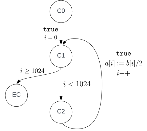
(b) C Program CFG. C0 is the entry node and EC is the exit node
